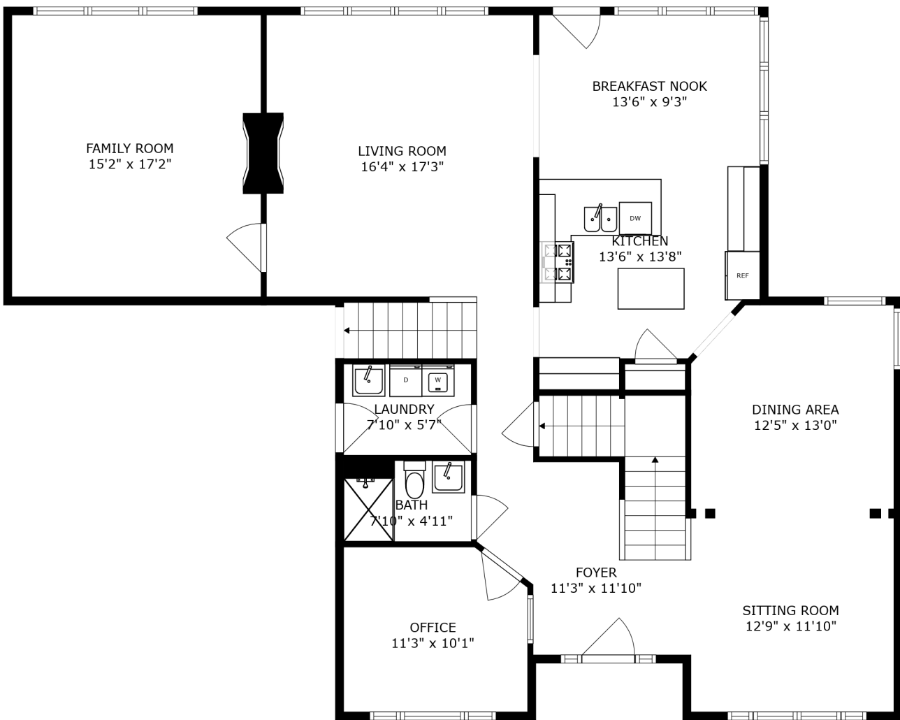
FLOOR 2
