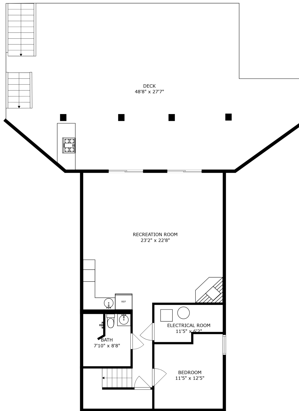
FLOOR 1
