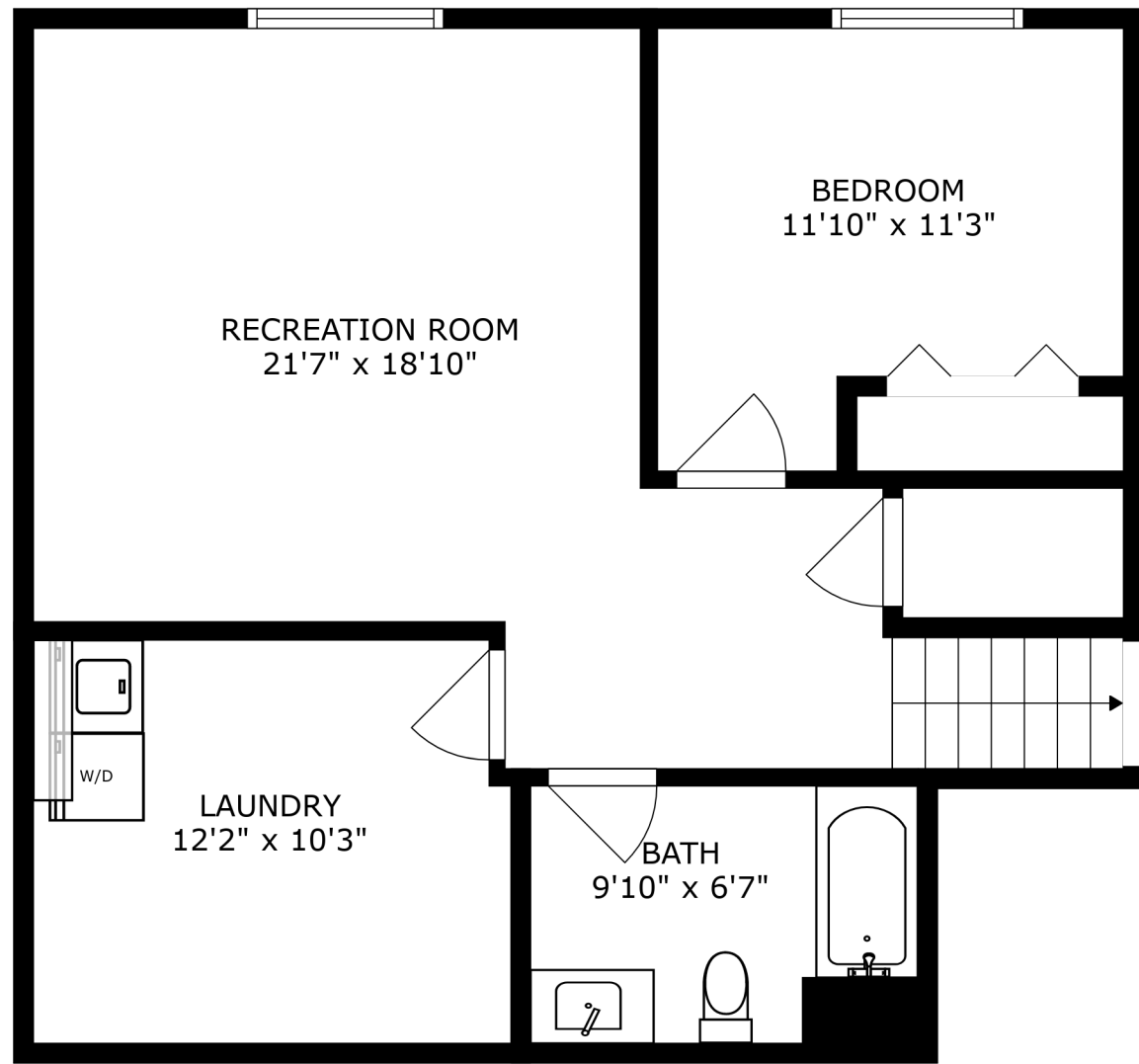
FLOOR 1
