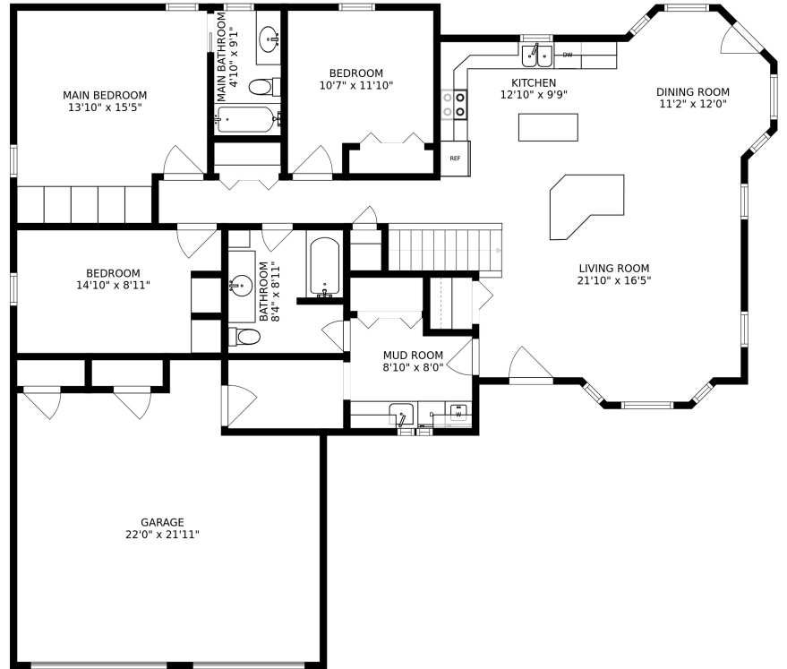
FLOOR 2
