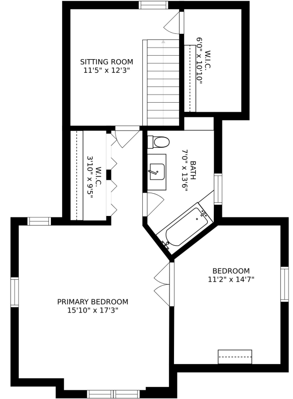
FLOOR 3
