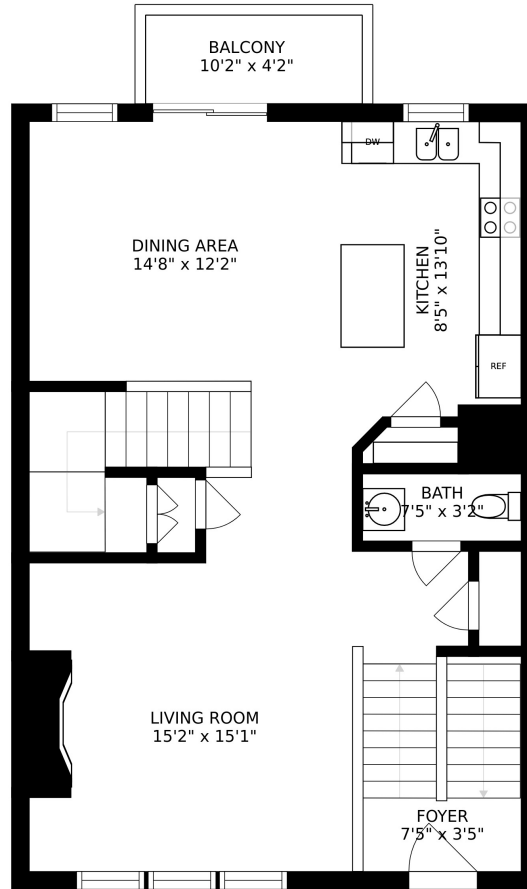
FLOOR 2
