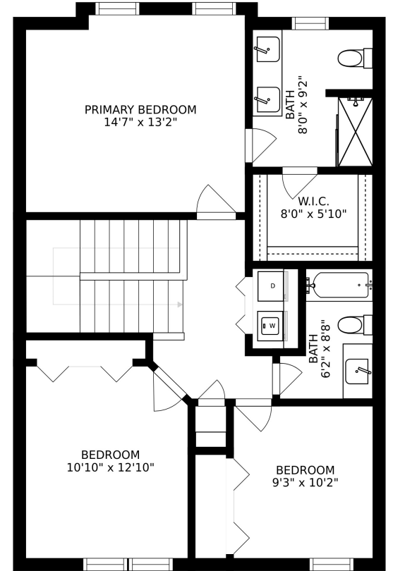
FLOOR 3
