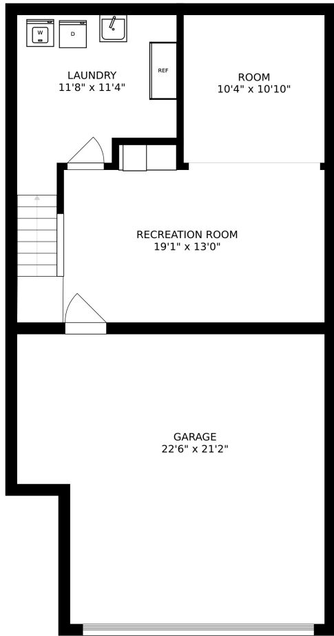
FLOOR 1
