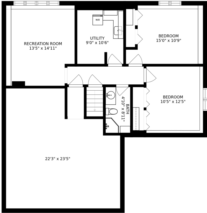
FLOOR 1
