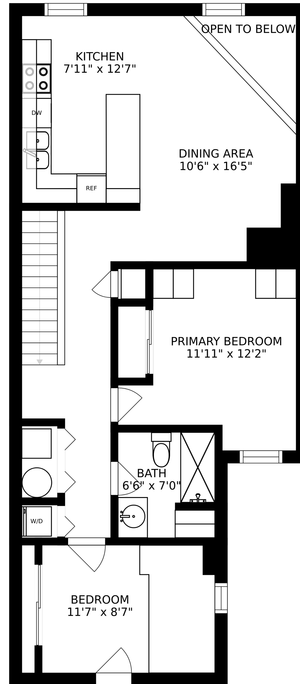
FLOOR 2
