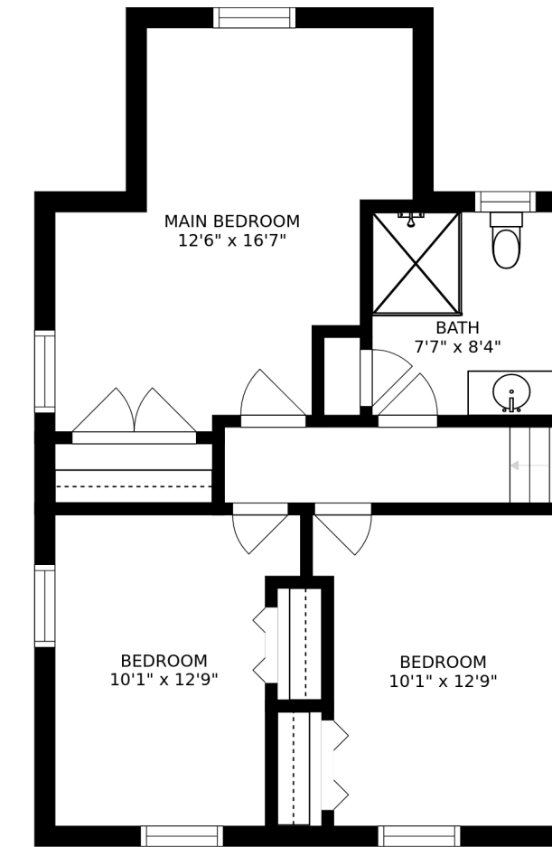
FLOOR 3
