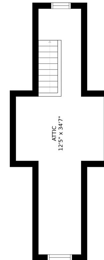
FLOOR 3
