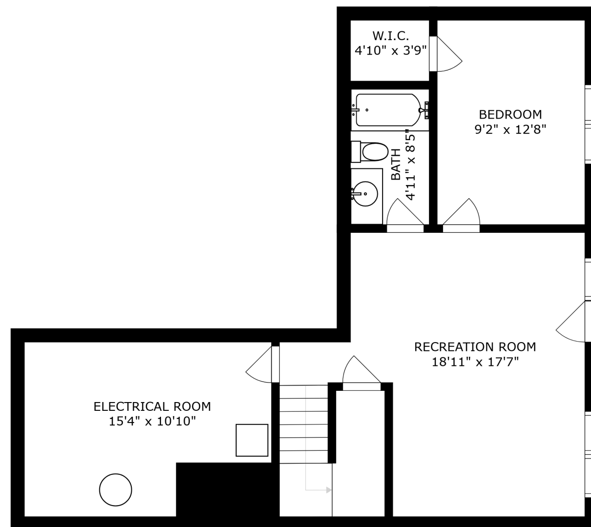
FLOOR 1
