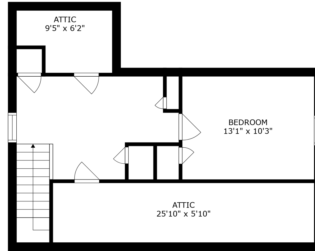
FLOOR 3
