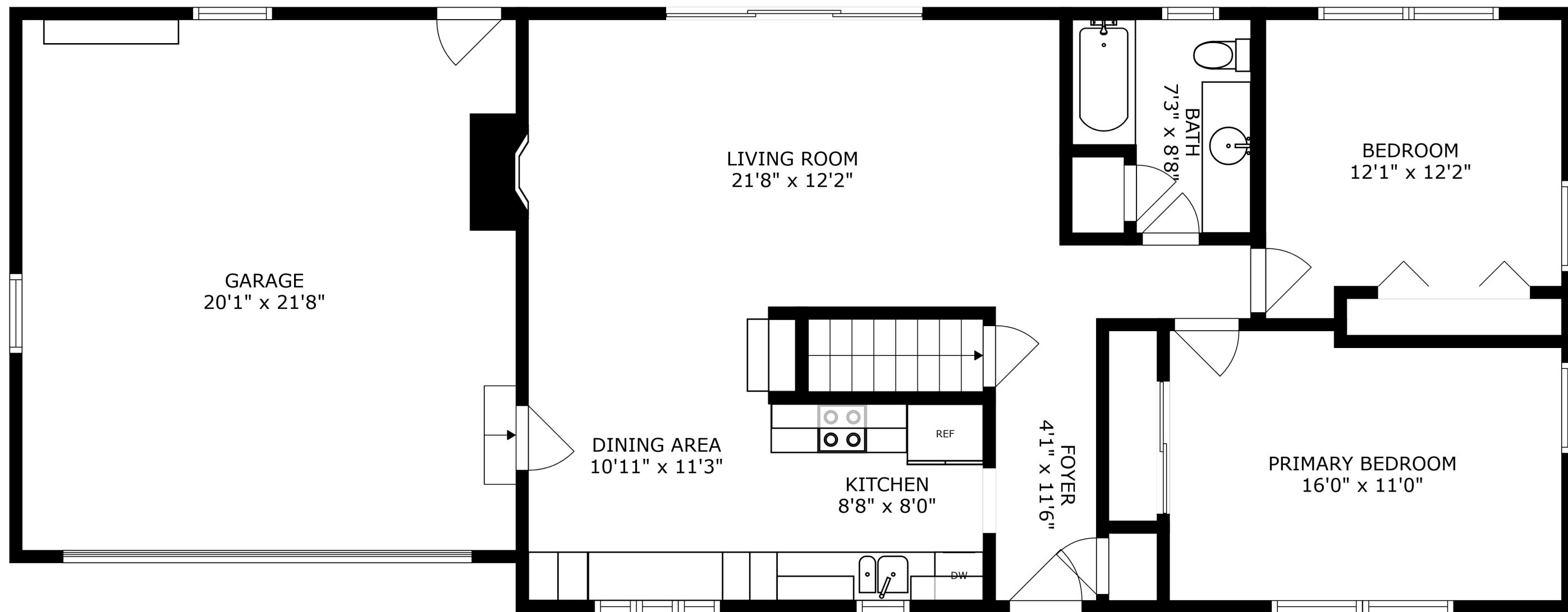
FLOOR 2
