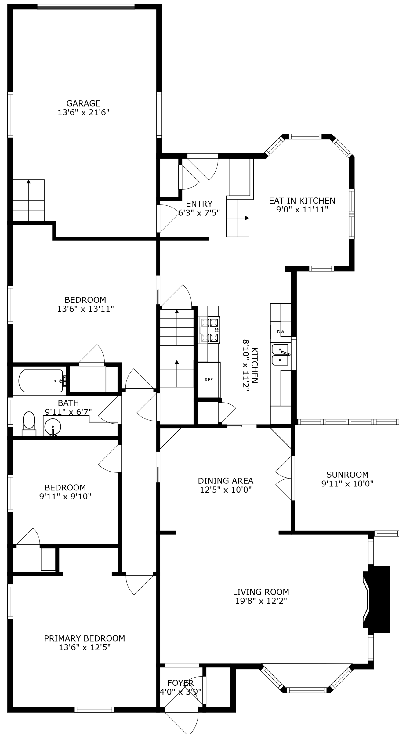
FLOOR 2
