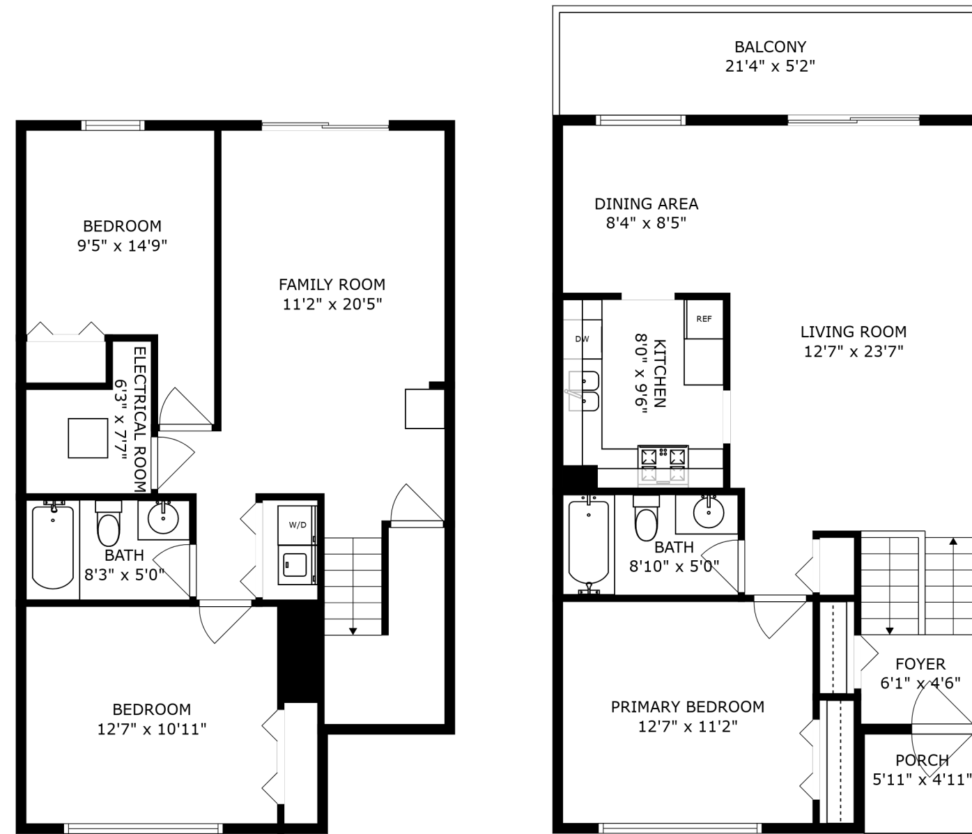
FLOOR 1
