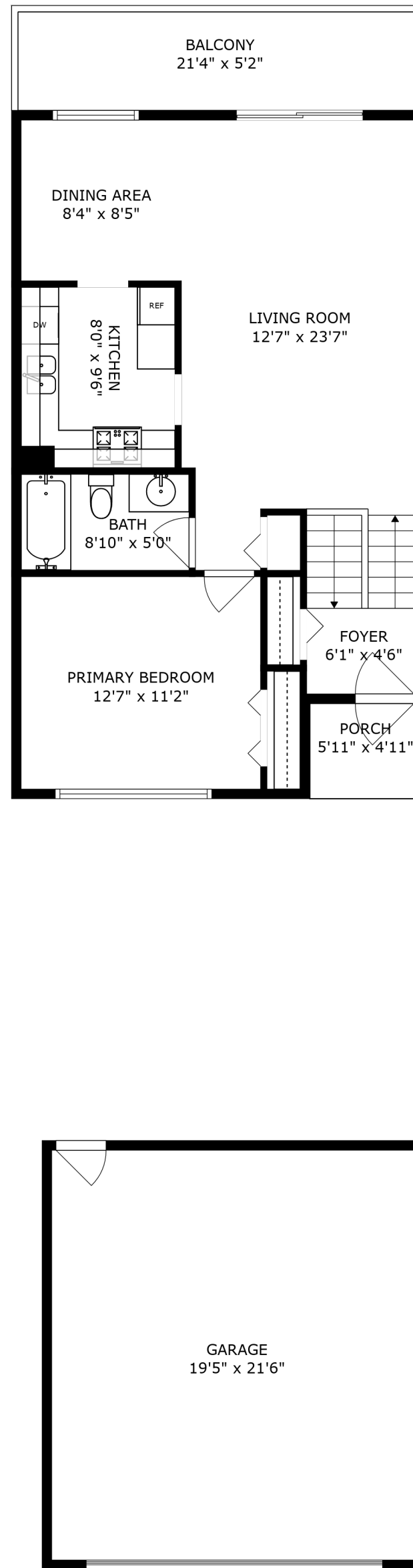
FLOOR 2
