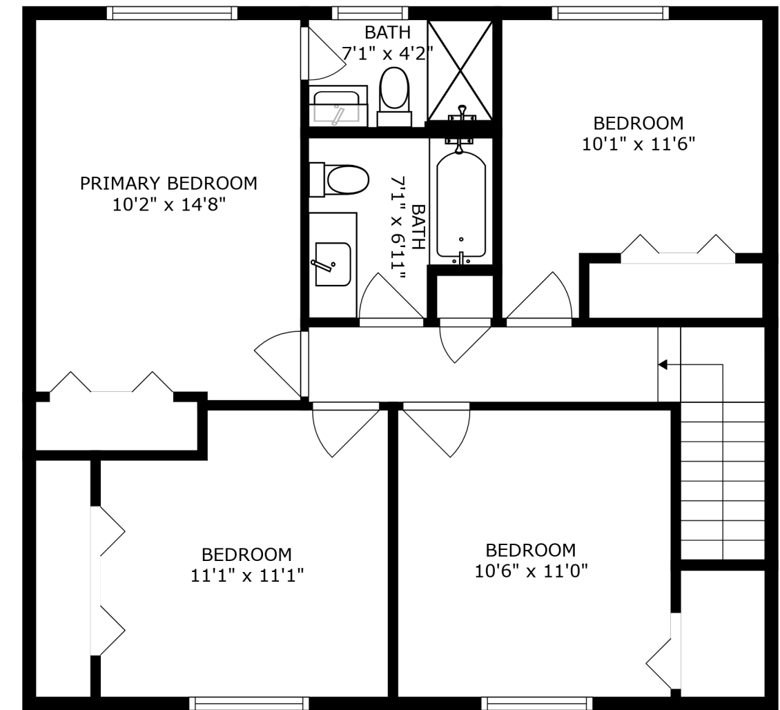
FLOOR 3
