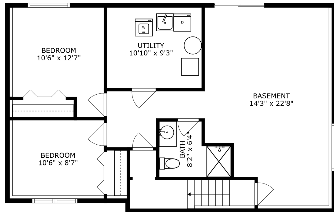
FLOOR 1
