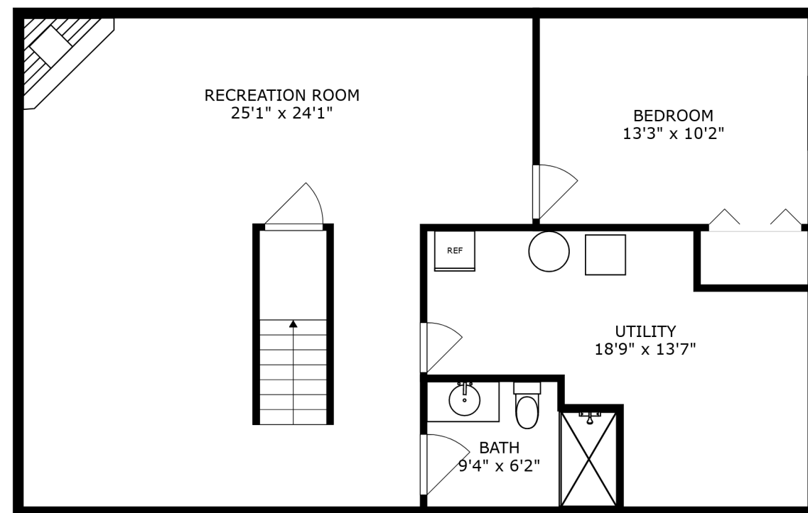
FLOOR 1
