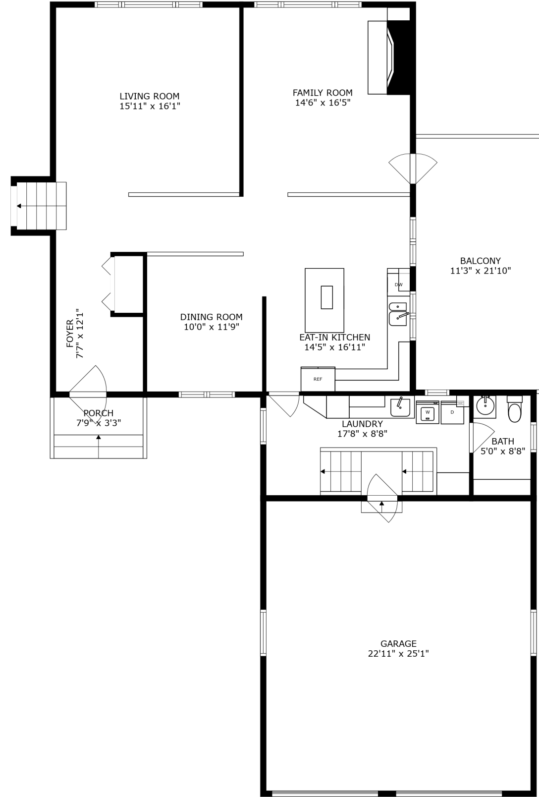
FLOOR 3
