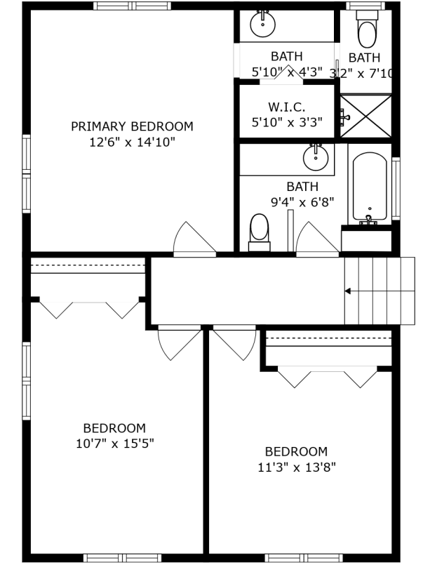
FLOOR 4
