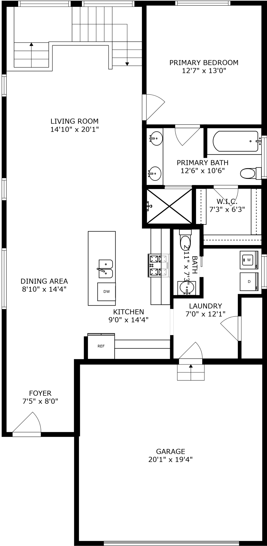
FLOOR 2
