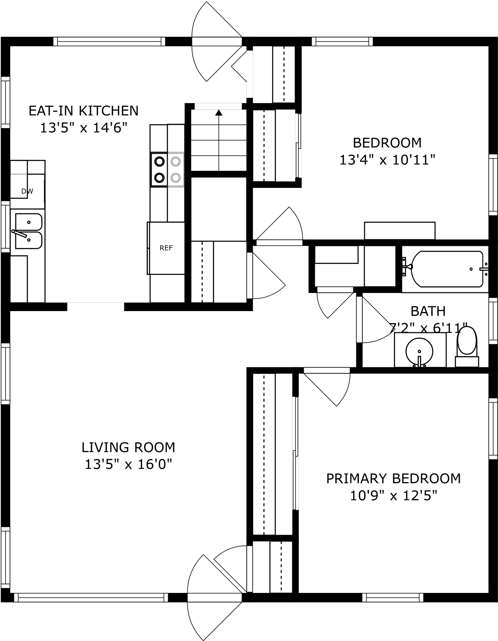
FLOOR 2
