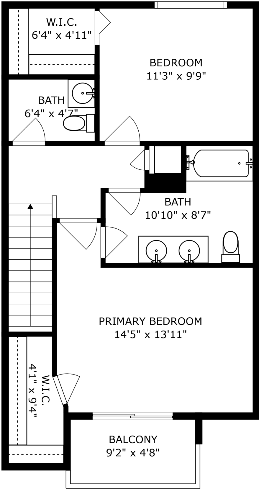
FLOOR 3
