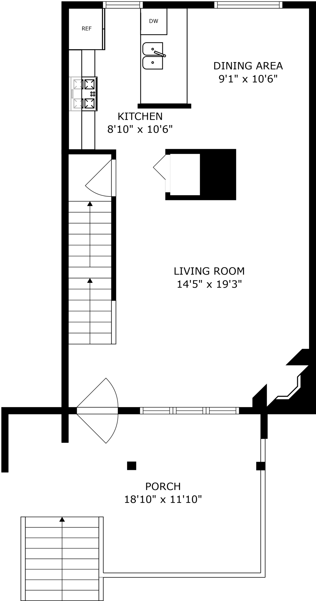
FLOOR 2
