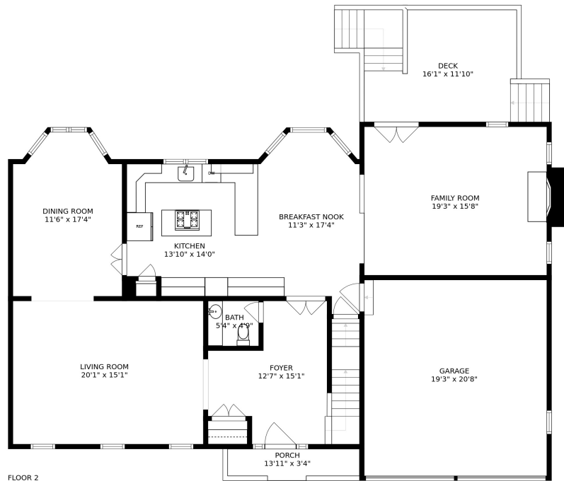
FLOOR 2
