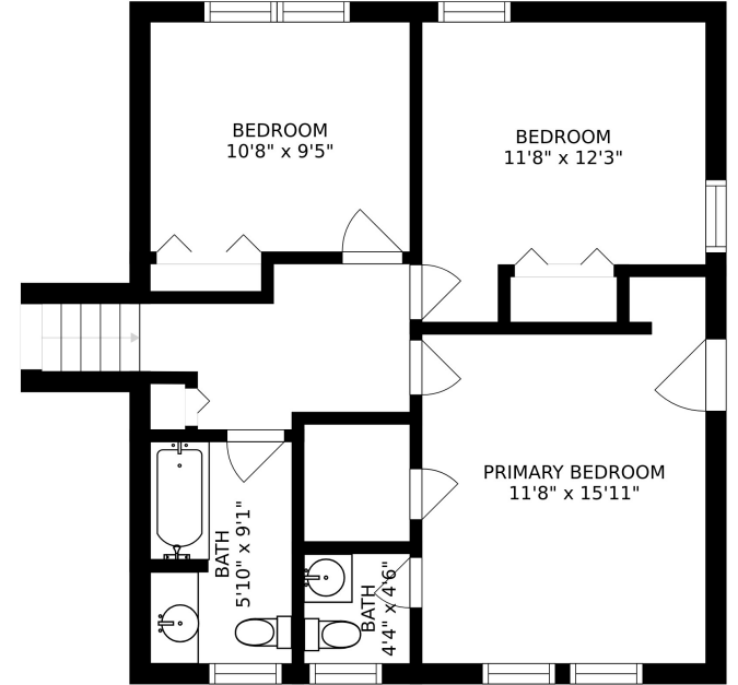
FLOOR 2
