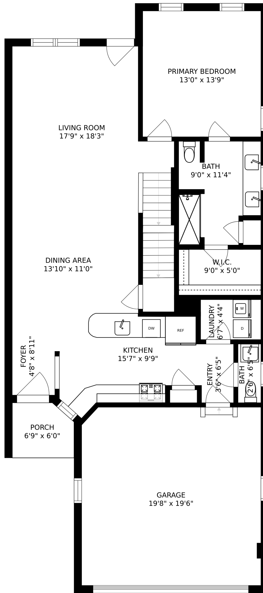
FLOOR 2
