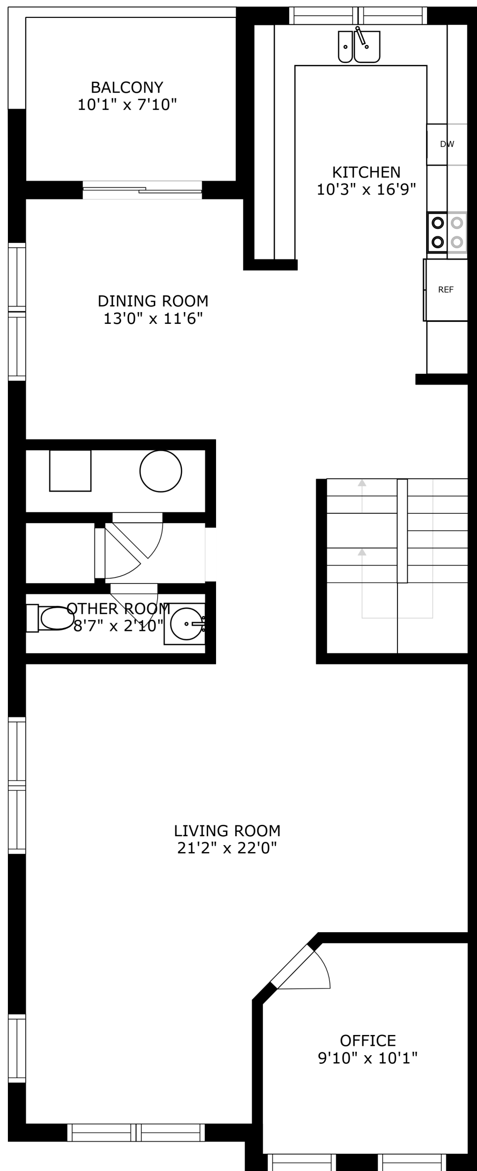
FLOOR 2
