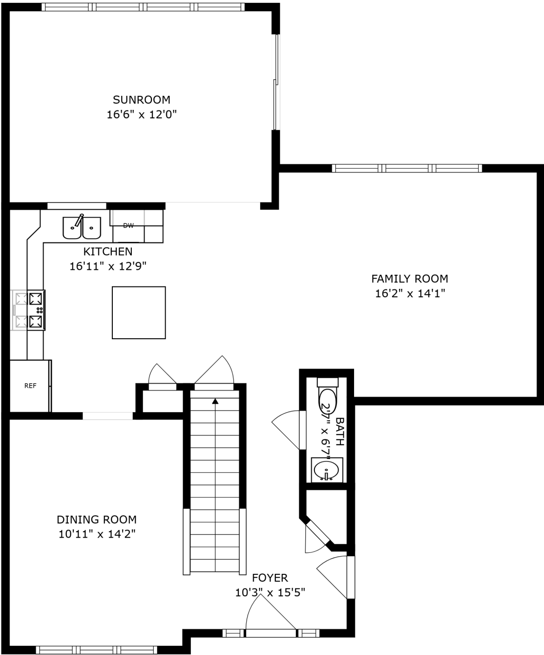
FLOOR 2
