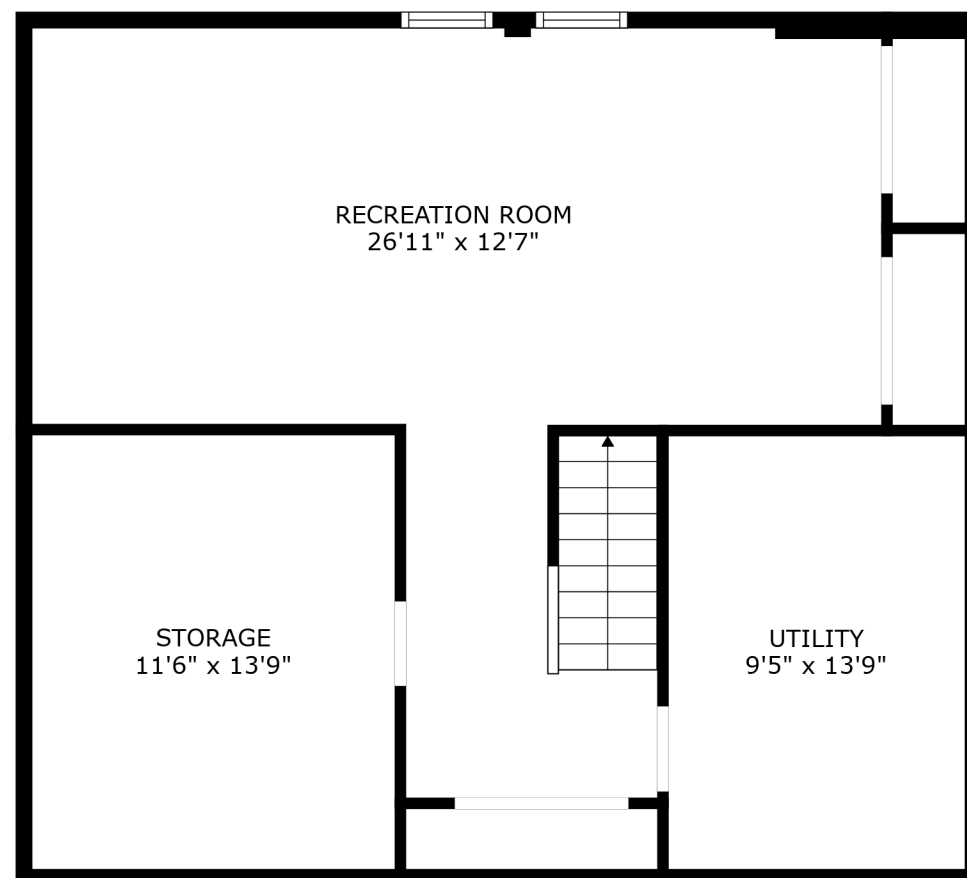
FLOOR 1
