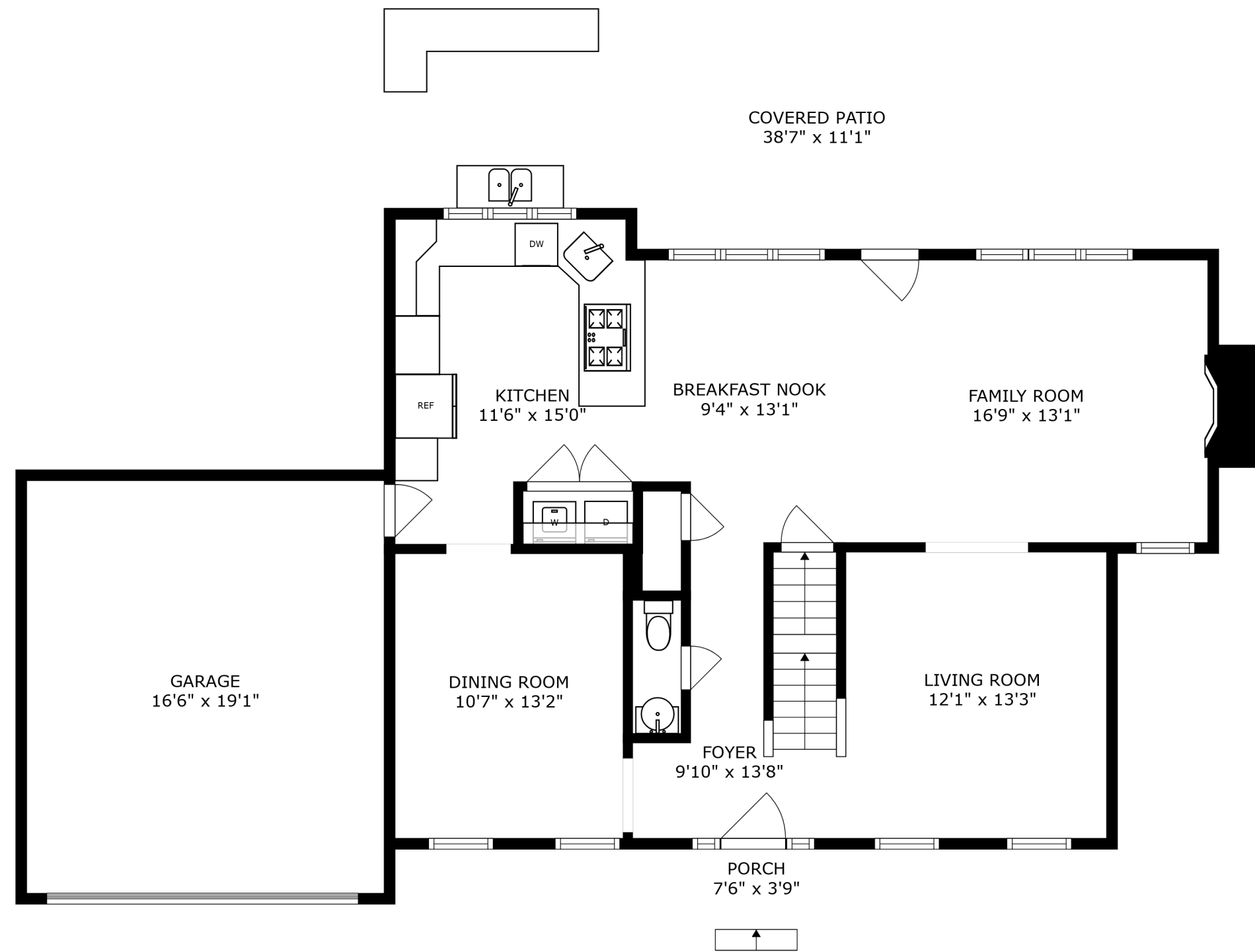
FLOOR 2
