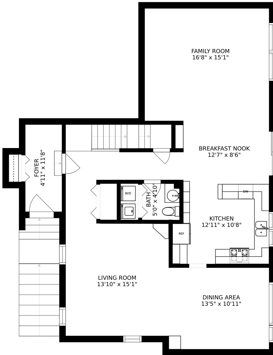
FLOOR 1
