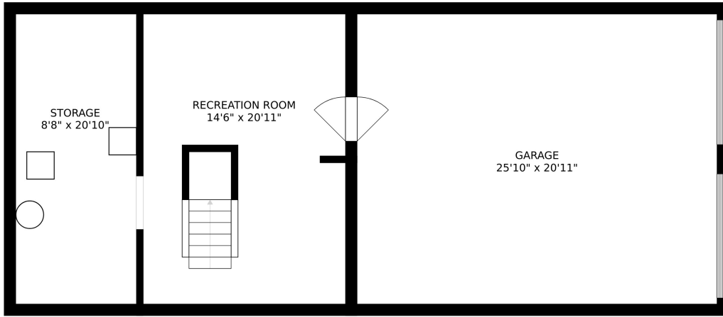
FLOOR 1
