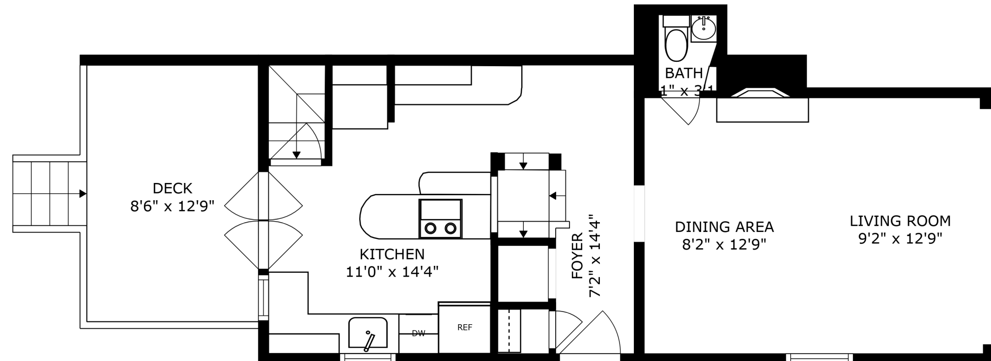
FLOOR 2
