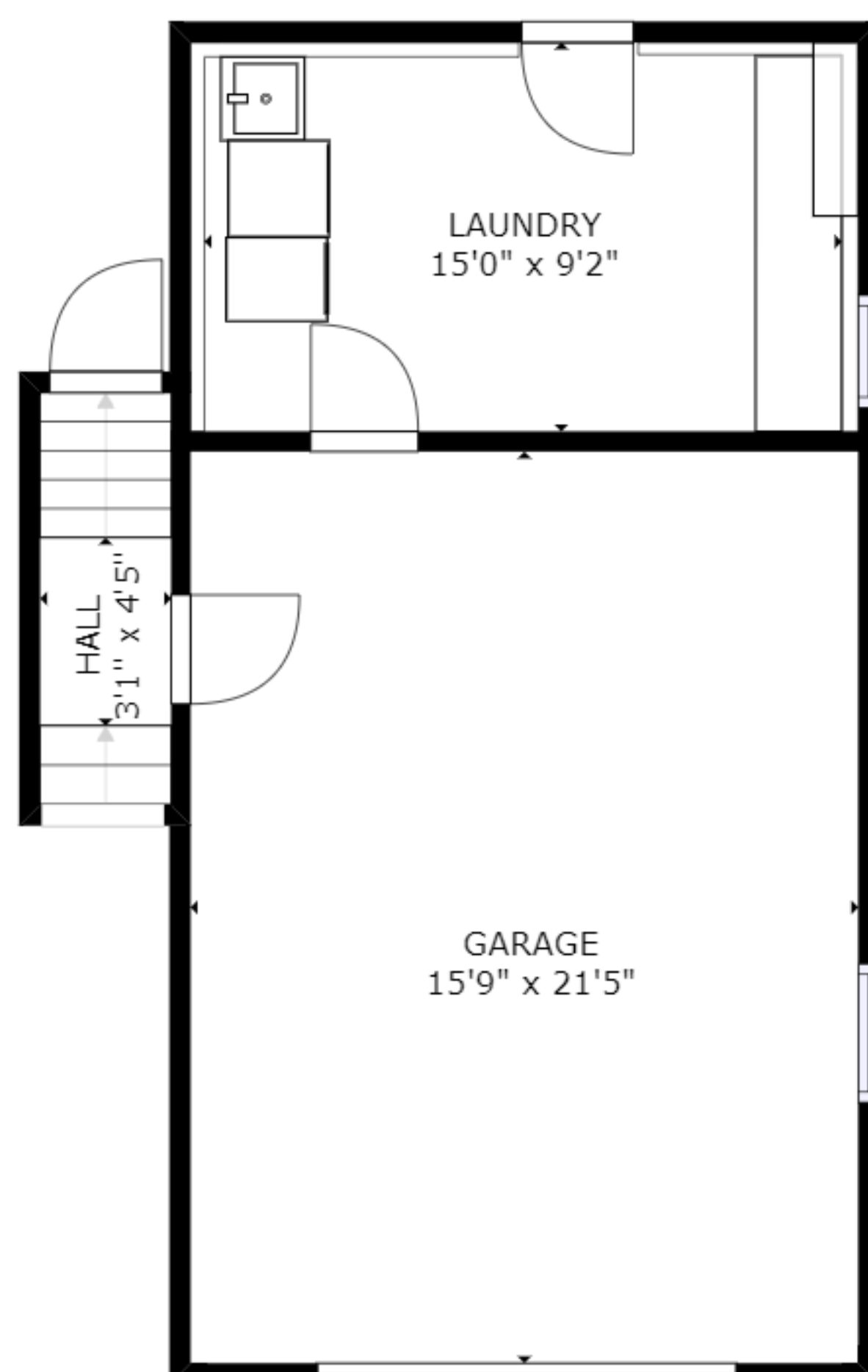
FLOOR 2
