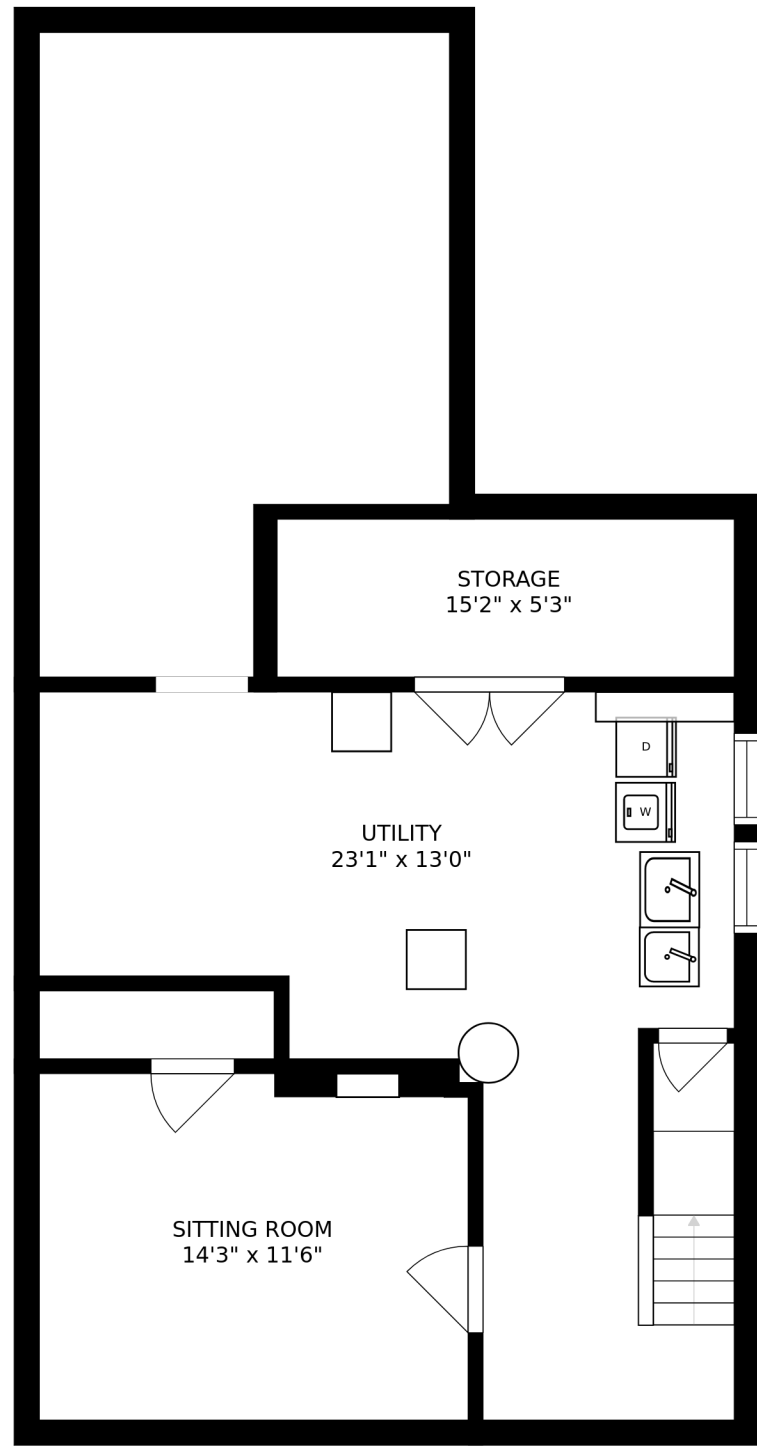
FLOOR 1
