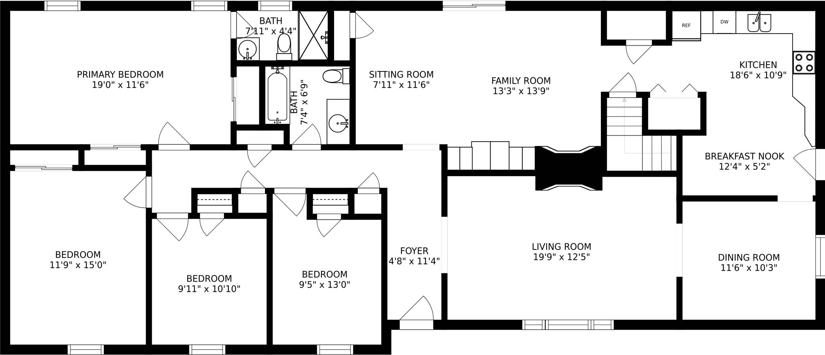
FLOOR 2
