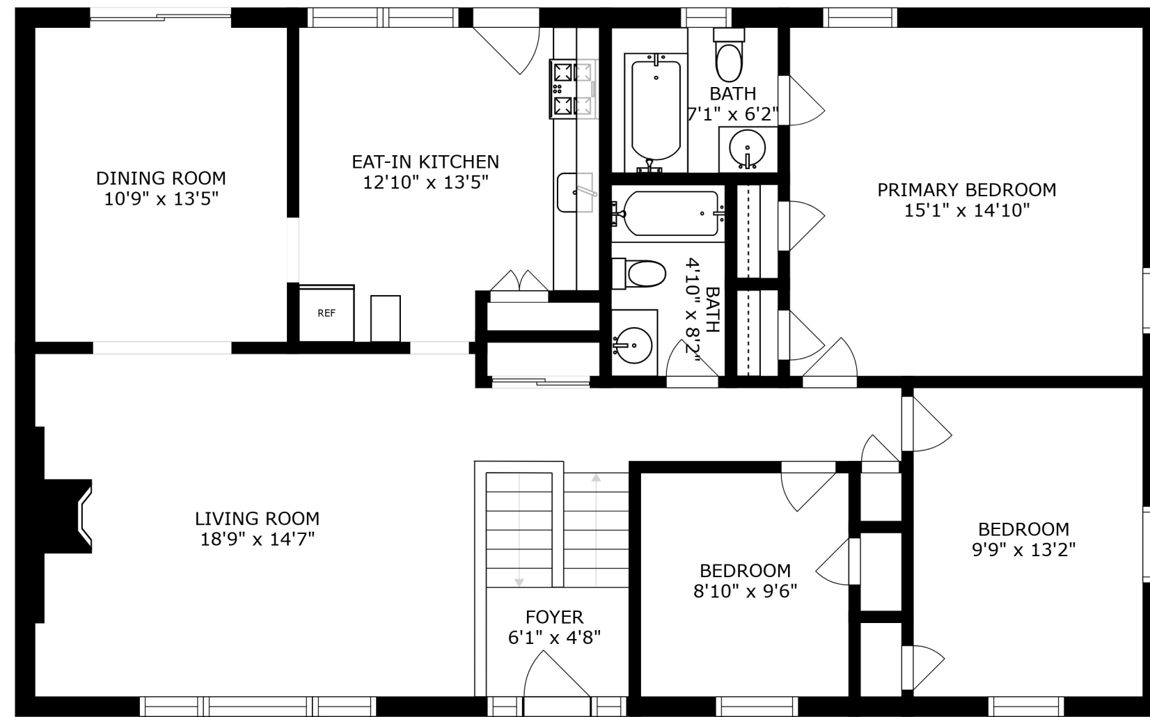
FLOOR 2
