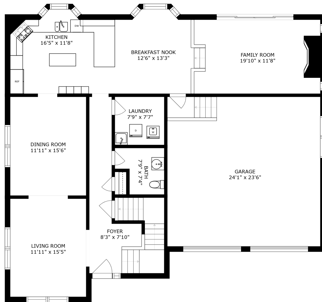
FLOOR 2
