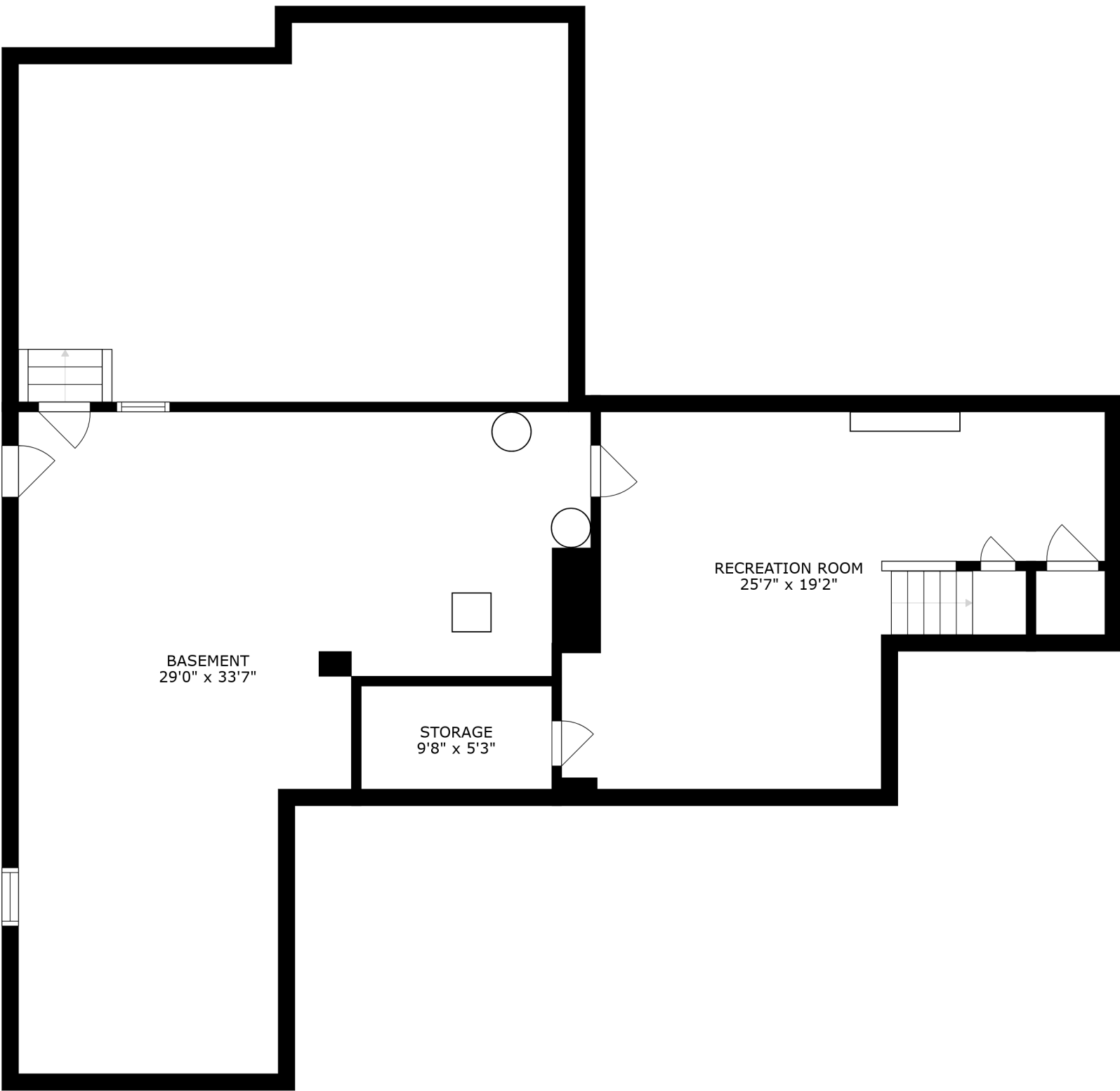
FLOOR 1
