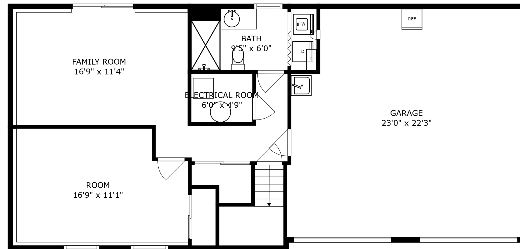
FLOOR 1
