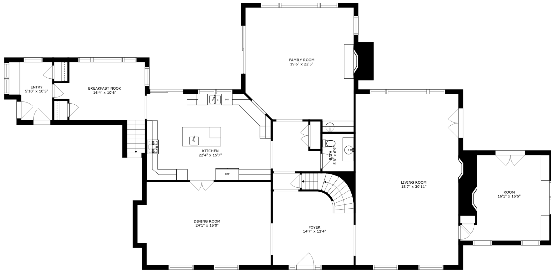
FLOOR 2
