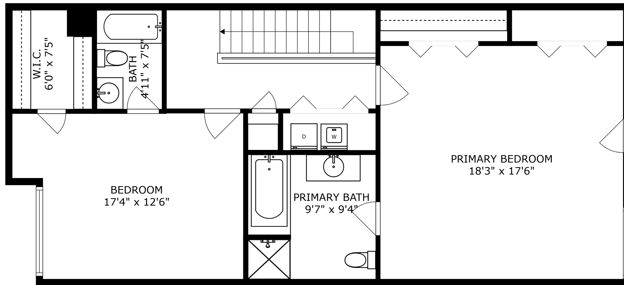
FLOOR 2
