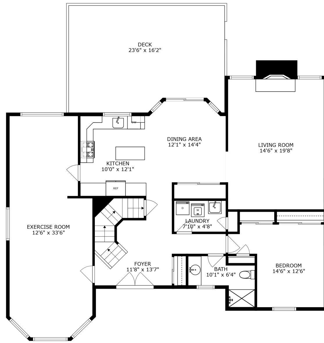
FLOOR 2
