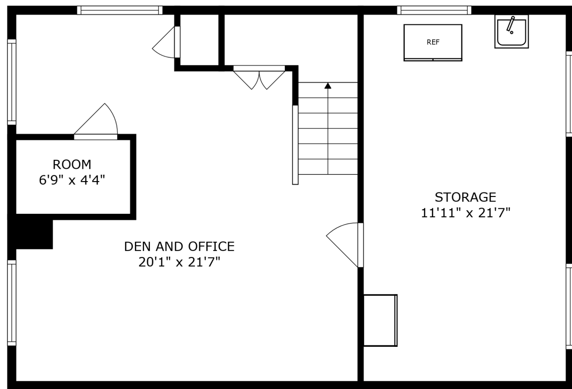
FLOOR 1
