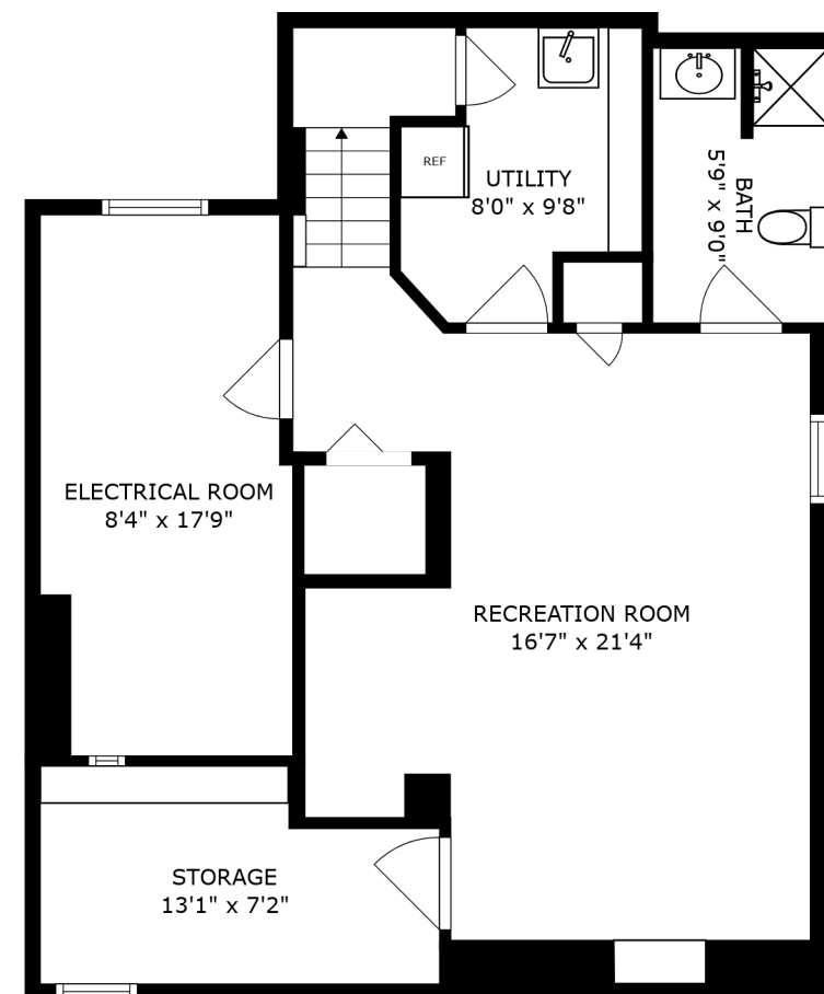
FLOOR 1
