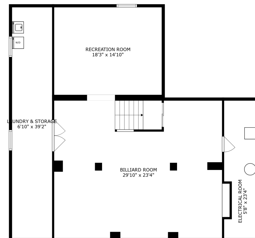
FLOOR 1
