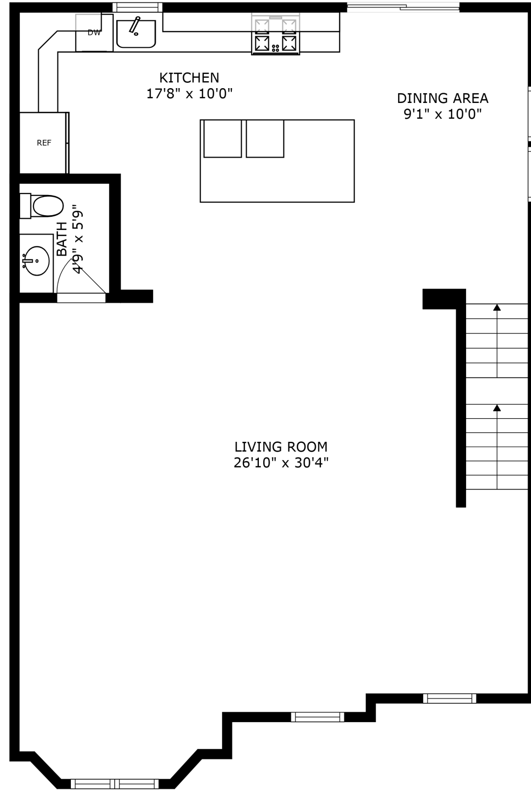
FLOOR 2
