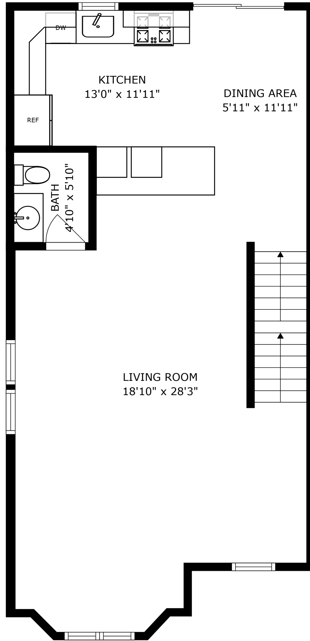
FLOOR 2
