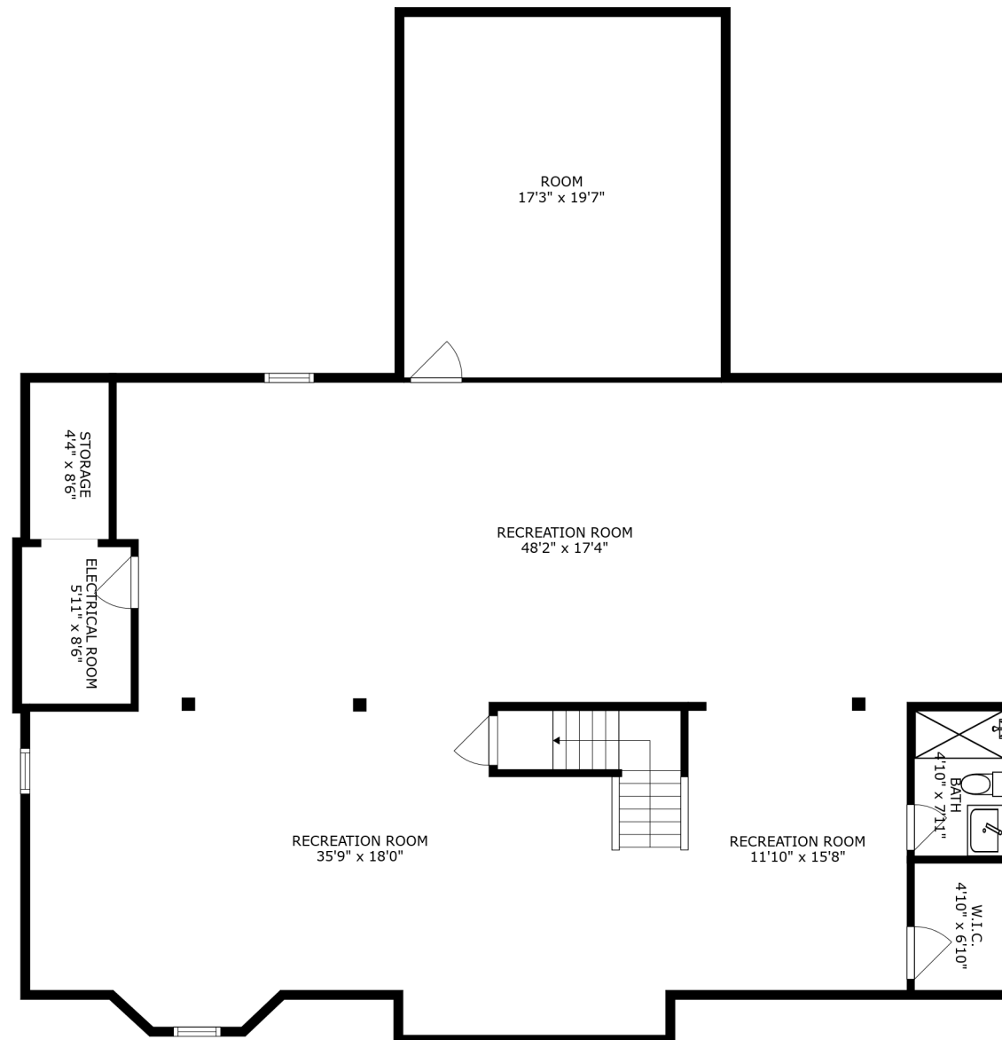
FLOOR 1
