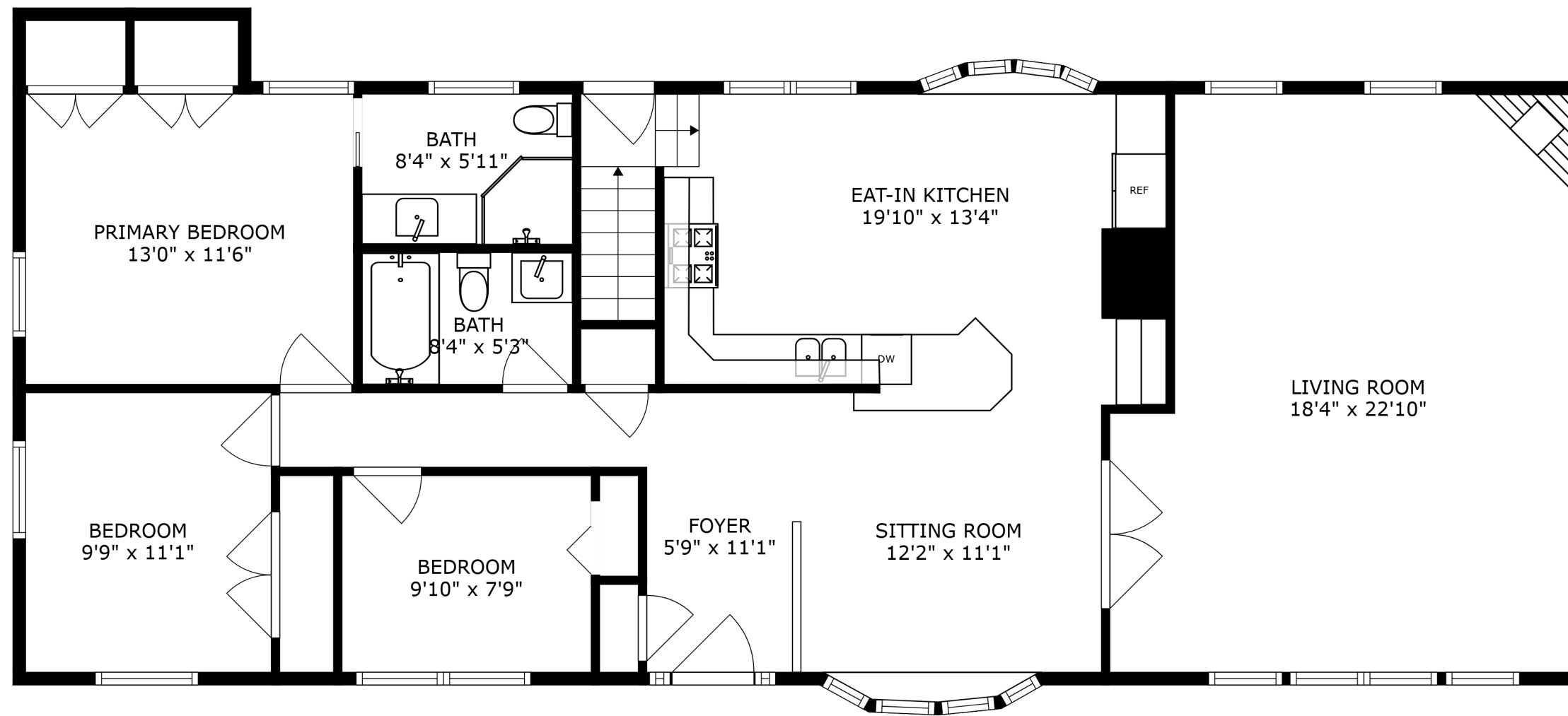
FLOOR 2
